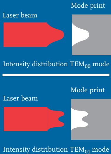
Fig. 4: Intensity distribution across the laser beam
