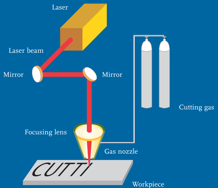
Fig. 1: Principles of a laser cutting system (schematic)
