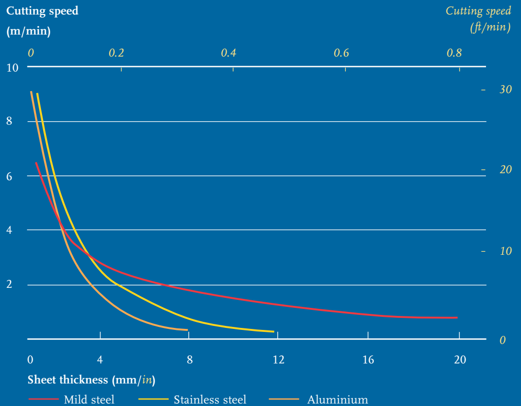
Fig. 2: Typical cutting rates with approx. 3 kW of laser power
