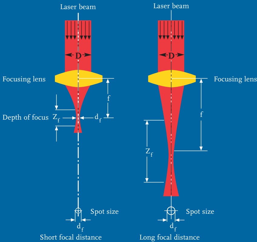
Fig. 3: Focusing a laser beam
