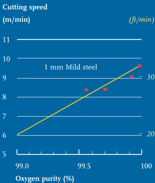
Fig. 9: Effect of oxygen purity on the cutting speed for 1 mm (0.04 in) mild steel using 800 W laser power and cutting oxygen pressure of 3 bar (44 psi)
